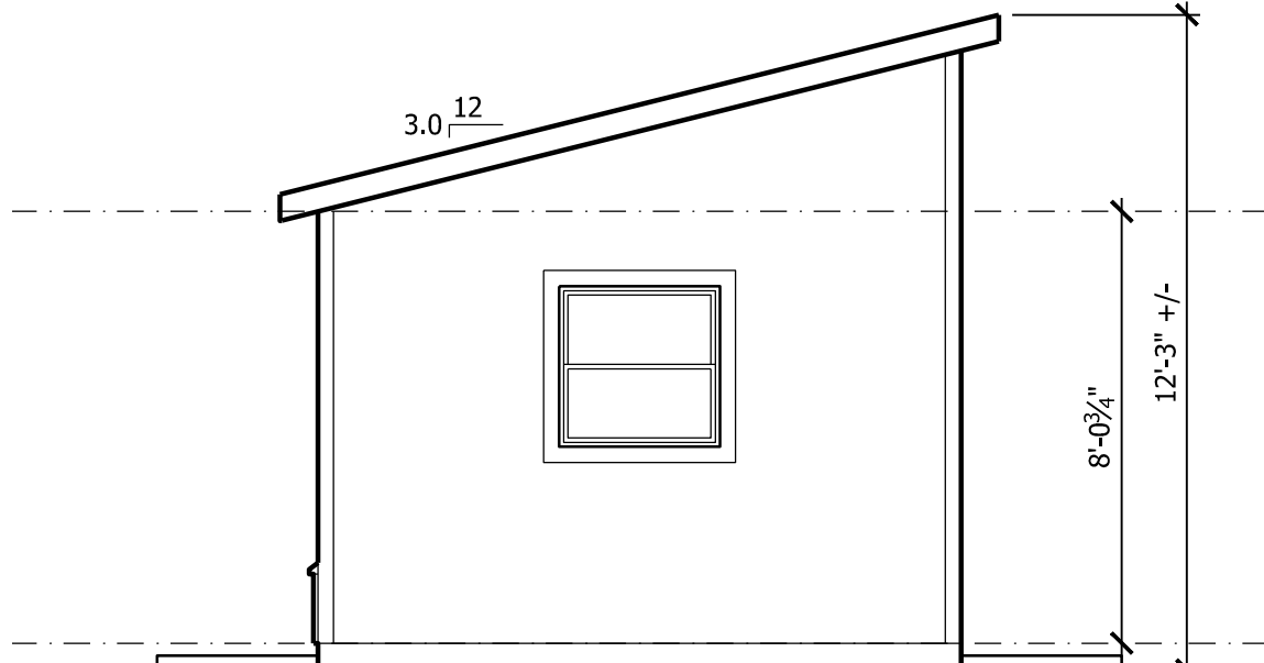
B2 RIGHT ELEVATION 1 1/4" = 1'-0"
