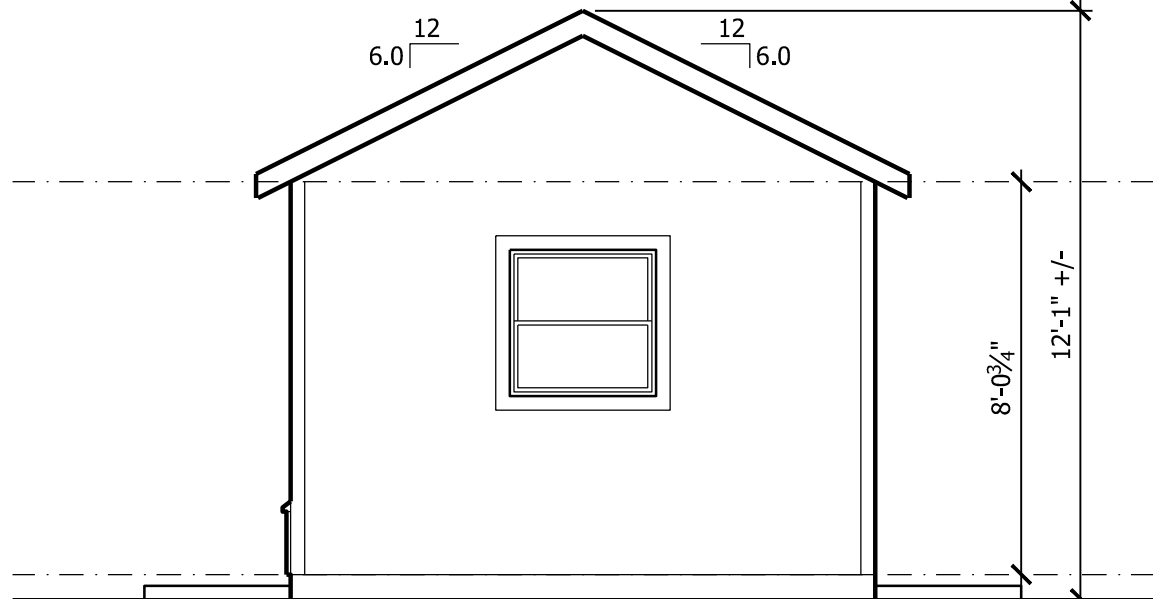
B RIGHT ELEVATION 1 1/4" = 1'-0"
