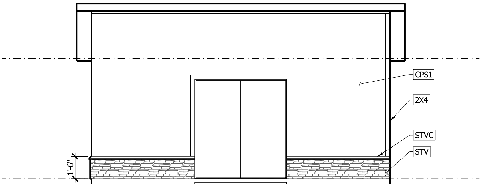
A2 FRONT ELEVATION 1 1/4" = 1'-0"
