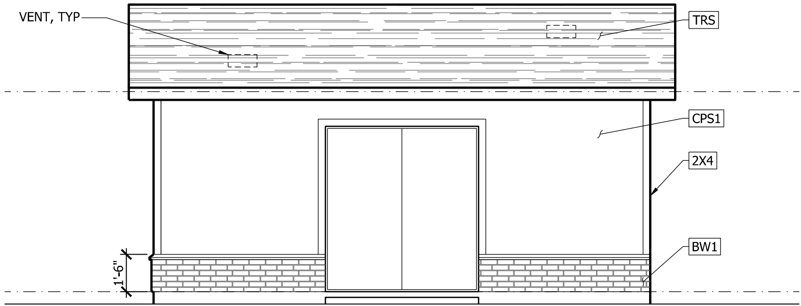
A FRONT ELEVATION 1 1/4" = 1'-0"
