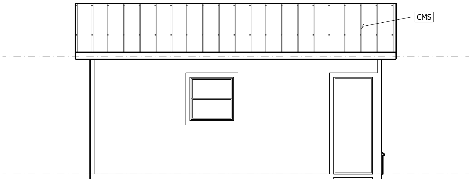
C2 REAR ELEVATION 1 1/4" = 1'-0"
